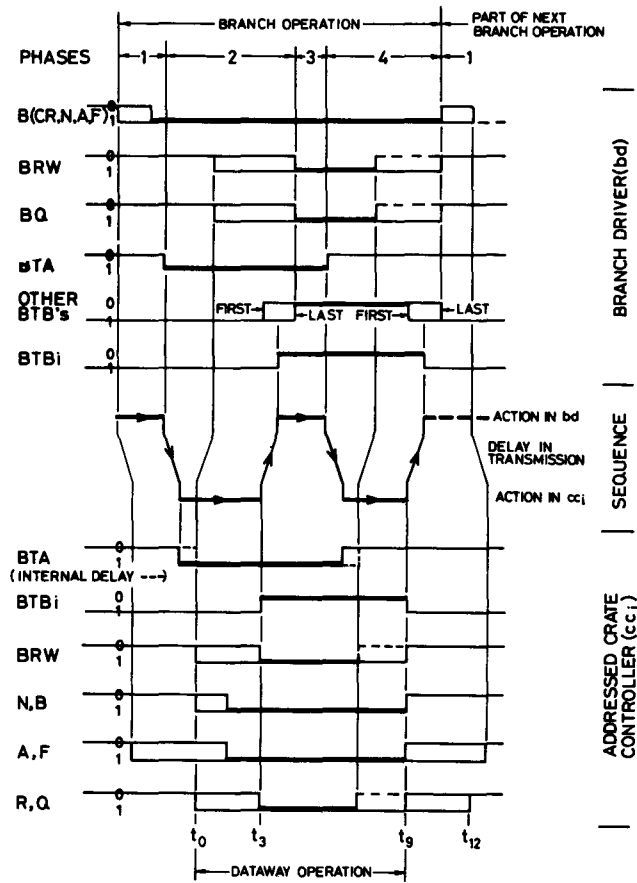
Fig.3. TIMING OF BRANCH READ OPERATION
