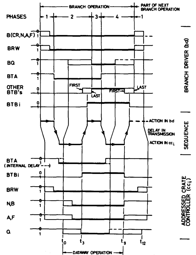
Fig. 4. TIMING OF BRANCH WRITE OPERATION
