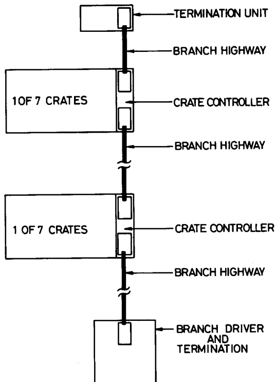
Fig. 1. CAMAC BRANCH: CHAIN CONFIGURATION
