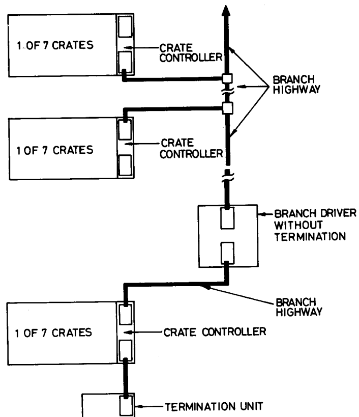
Fig. 2. CAMAC BRANCH: EXAMPLE OF AN ALTERNATIVE CONFIGURATION
