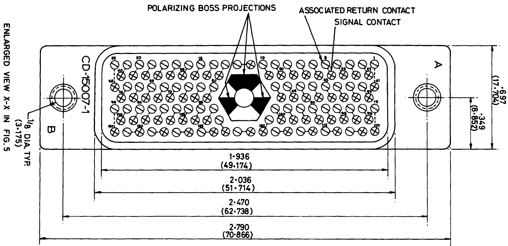
Fig. 6. BRANCH HIGHWAY PORTS: CONTACT LAYOUT. (FRONT VIEW OF FIXED CONNECTOR)
