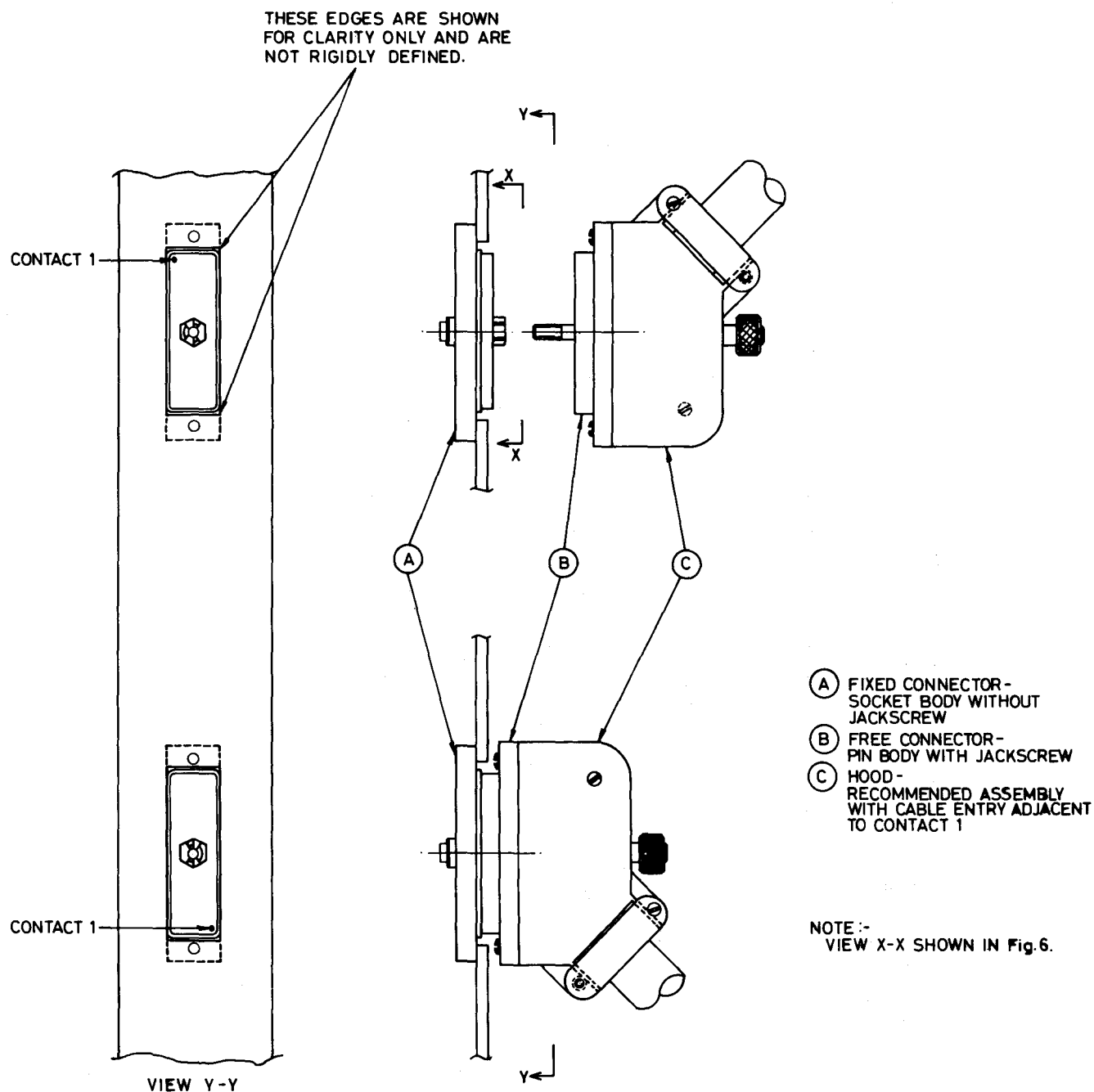
Fig. 5. BRANCH HIGHWAY PORTS: ARRANGEMENT OF CONNECTORS ON CRATE CONTROLLERS
