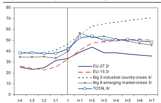
Graph III.3.7: Gross public debt in crises episodes (% of GDP) 1/
