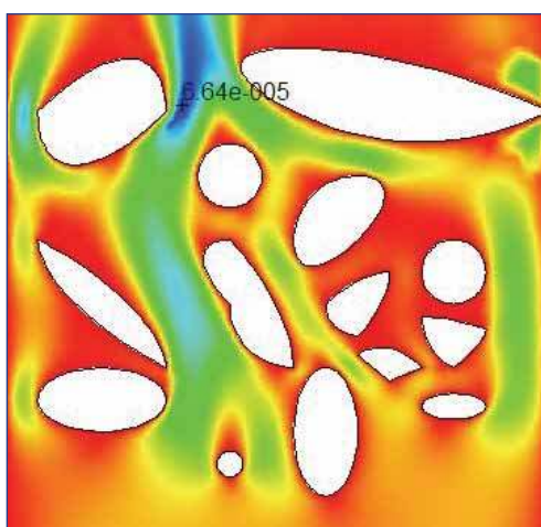
Computed velocity pattern inside a 2D porous microstructure (solid matrix in white). Maximum and minimum velocity (m/s) is indicated
