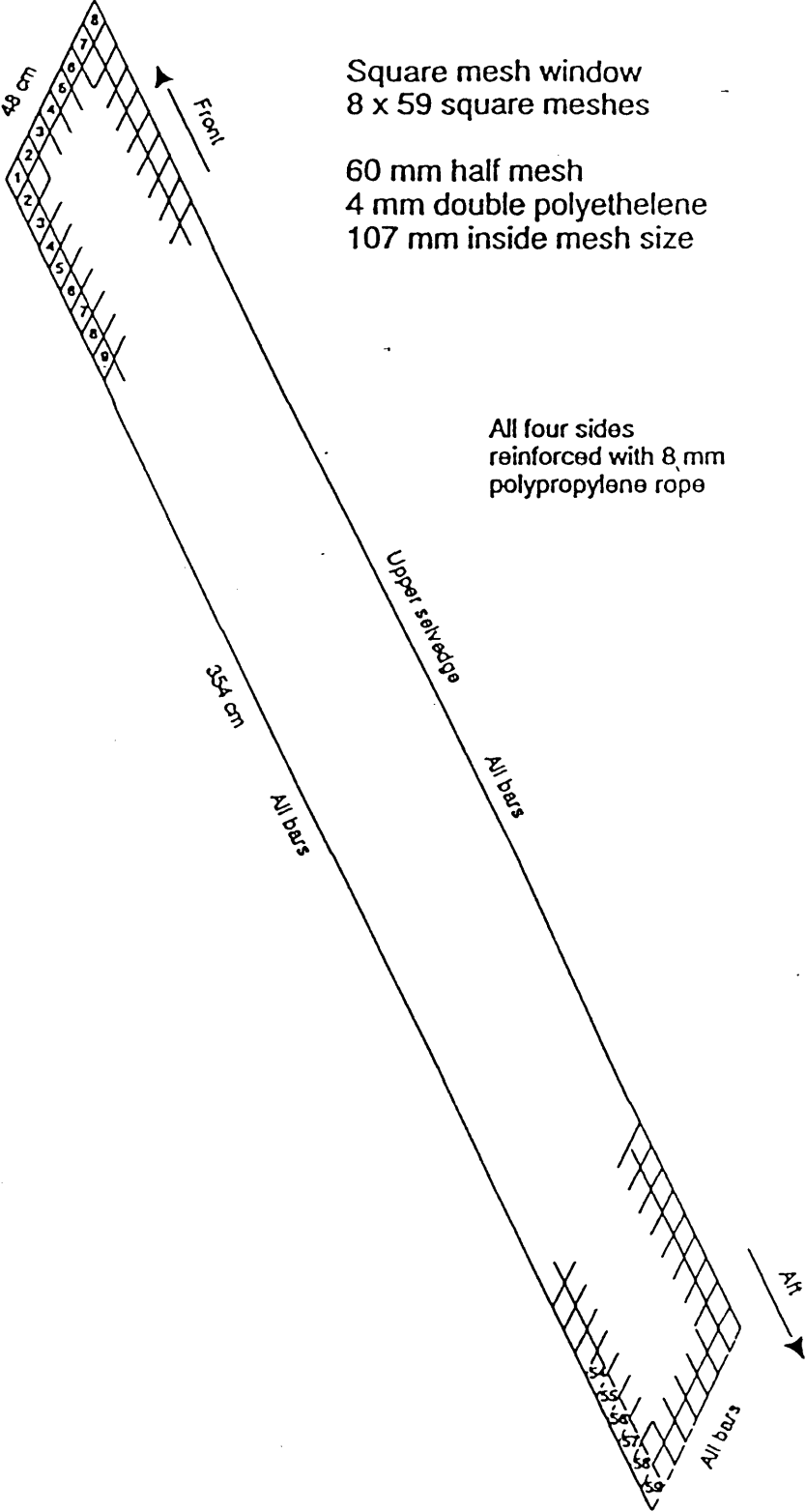
Figure 2 Netting in the square mesh windows A suggested specification
