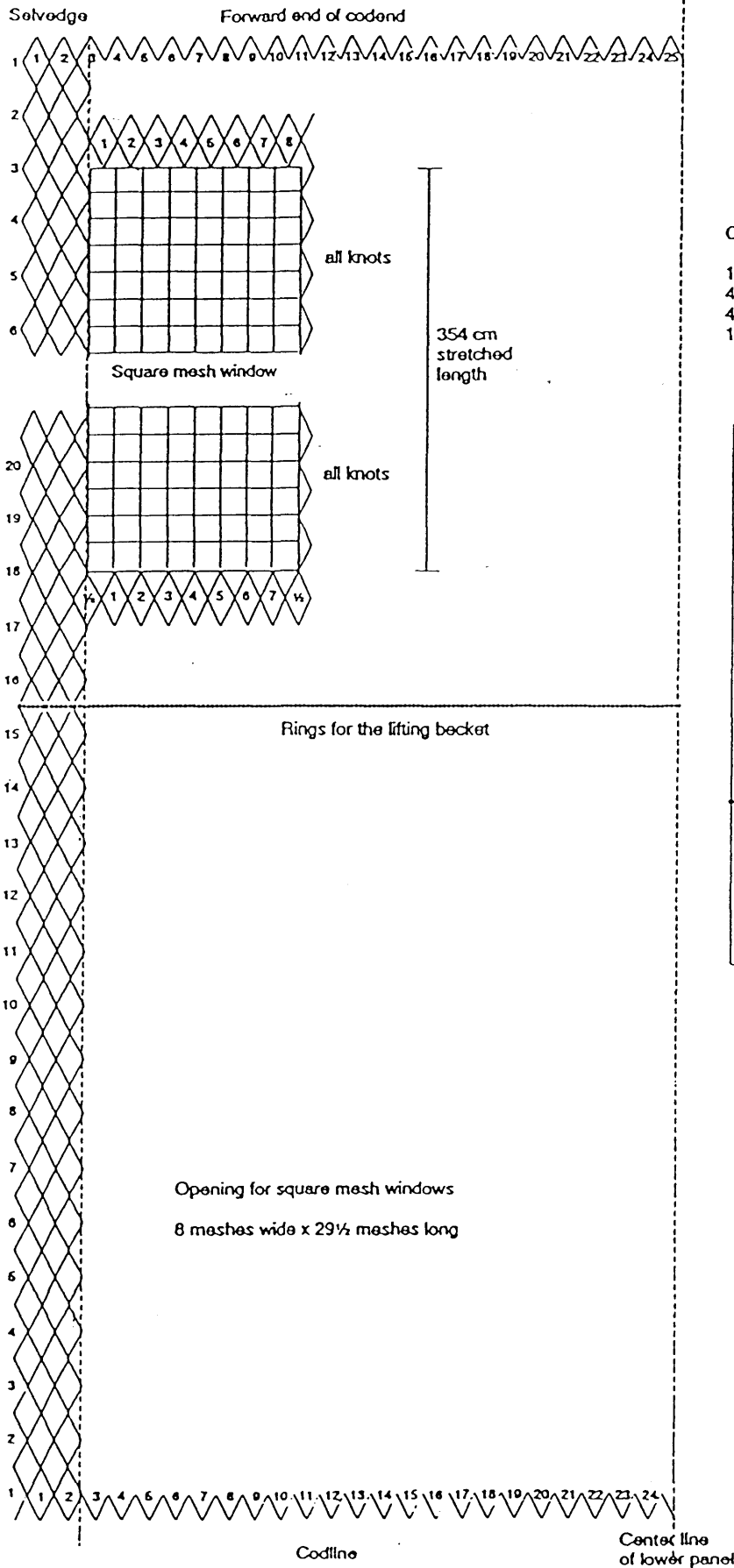
Figure 3 Inserting the window in the codend A suggested specification
