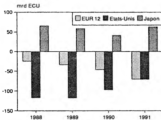
Gr. 1.2 - Balances commerciales
